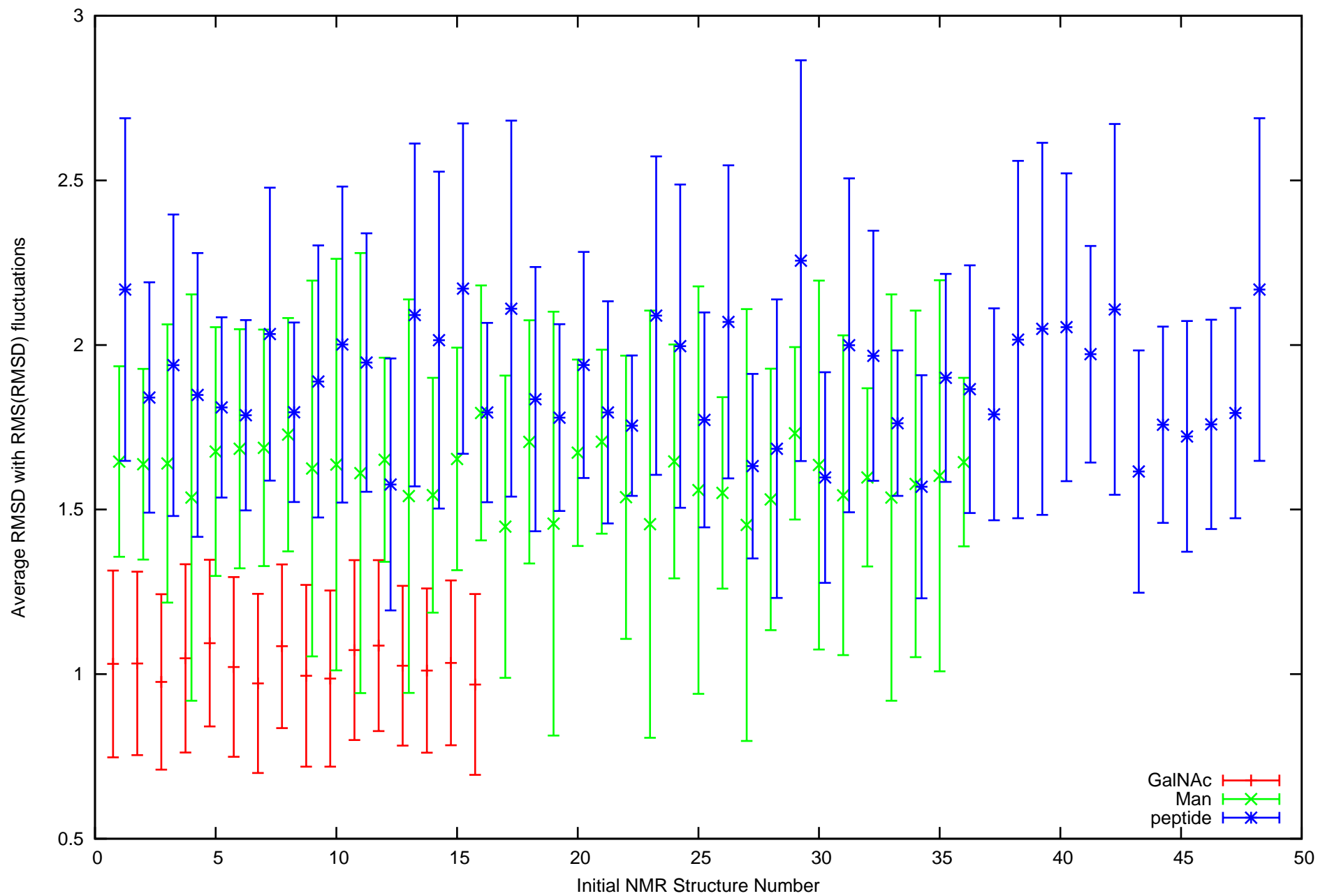
Backbone atoms CA, C, O, N, H in THR residues
