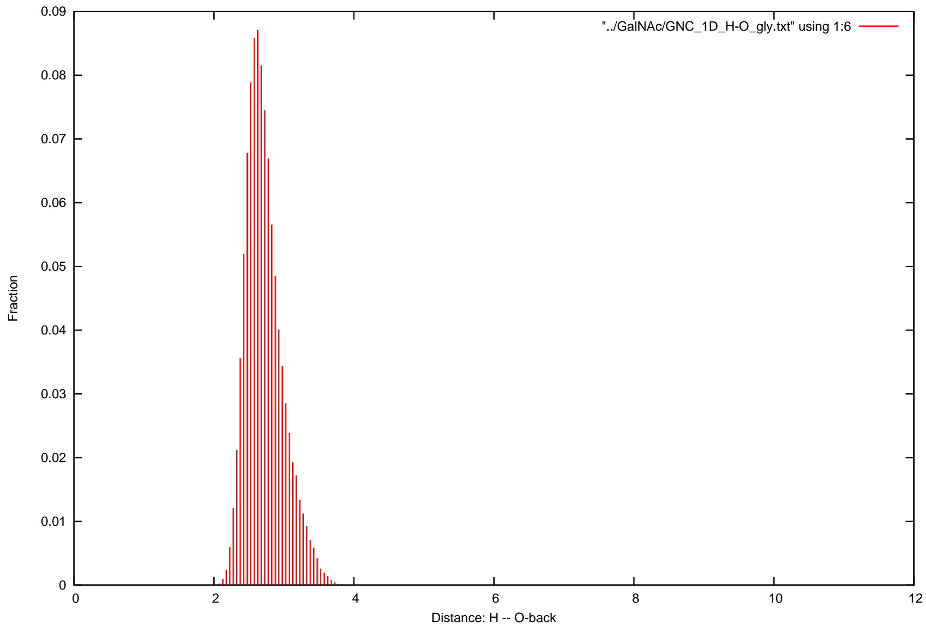
Normalized fraction over all simulations, all four GalNAc's
