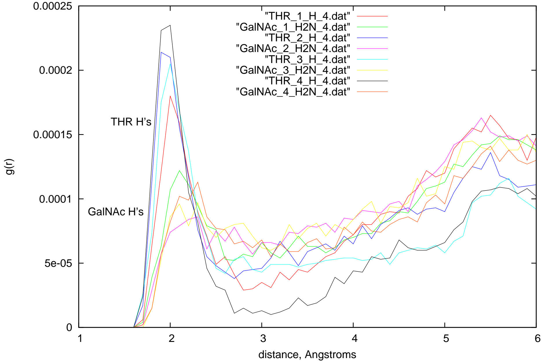
radial distributions for the relevant hydrogens to water O
