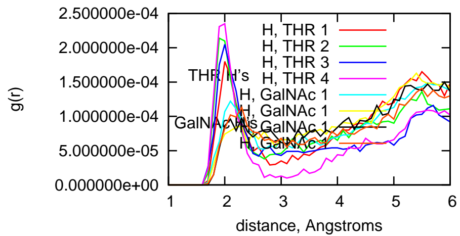
Radial distributions of water oxygen in run 4
